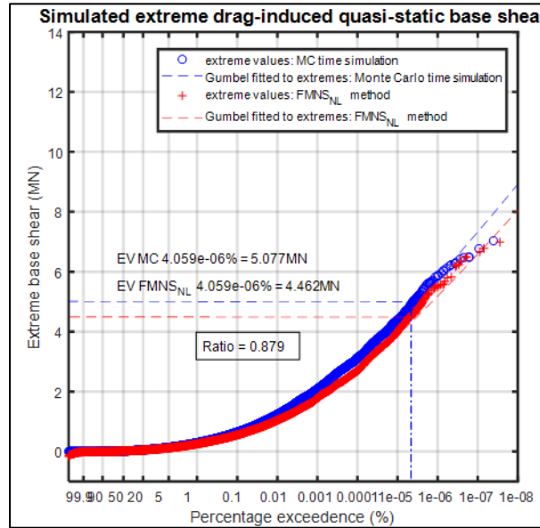
Figure 3. Comparison of Long-term Probability Distribution of Extreme Response Values From Monte Carlo Time Simulation and FMNS NL Methods, 1000 Response Records, Drag-induced Quasi-Static Base Shear, Current = 0.00 m/sec
