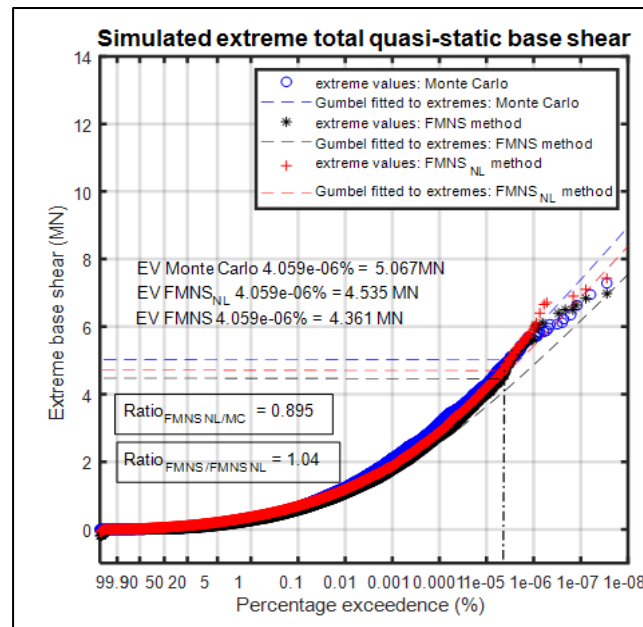
Figure 8. Comparison of Long-term Probability Distribution of Extreme Response Values From Monte Carlo Time Simulation, FMNS And FMNS NL Methods, 1000 Response Records, Total Quasi-Static Base Shear, Current = 0.00 m/sec
