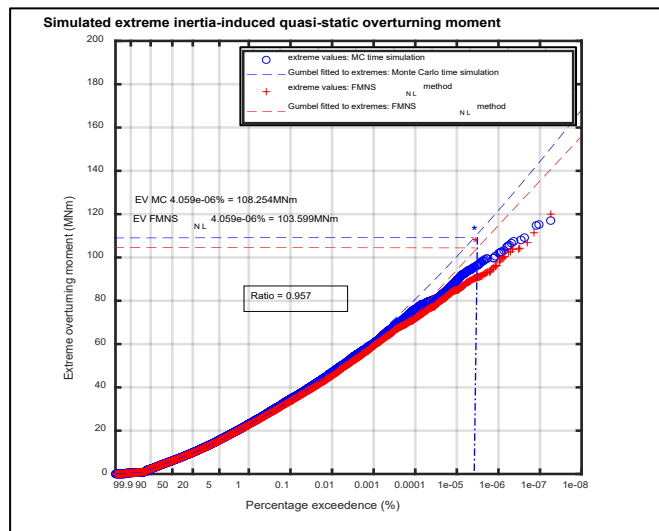
Figure 2. Comparison of Long-term Probability Distribution of Extreme Response Values From Monte Carlo Time Simulation and FMNS NL Methods, 1000 Response Records, Inertia-induced Quasi-Static Overturning Moment, Current = 0.00 m/sec
