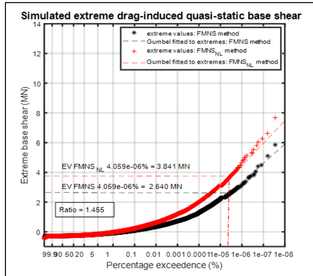
Figure 7. Comparison of Long-term Probability Distribution of Extreme Response Values From FMNS and FMNS NL Methods, 1000 Response Records, Drag-Induced Quasi-Static Base Shear, Current = -0.90 m/sec
