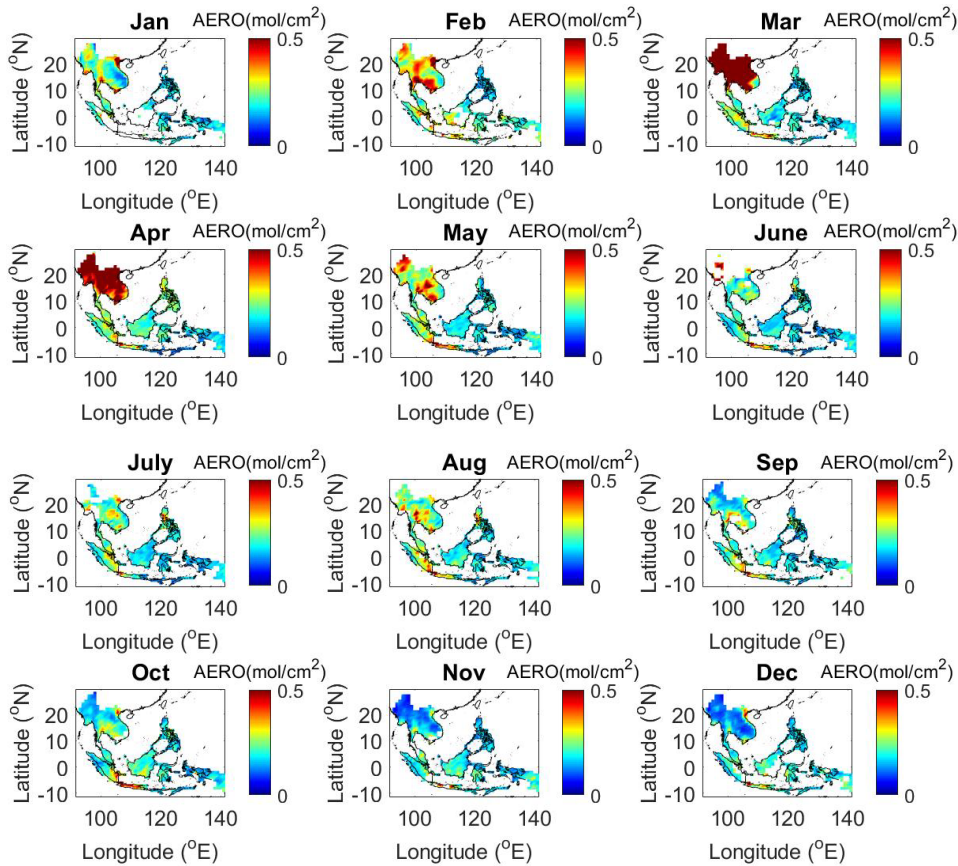
Figure 8. Aerosol pollution mapping from 2021.
