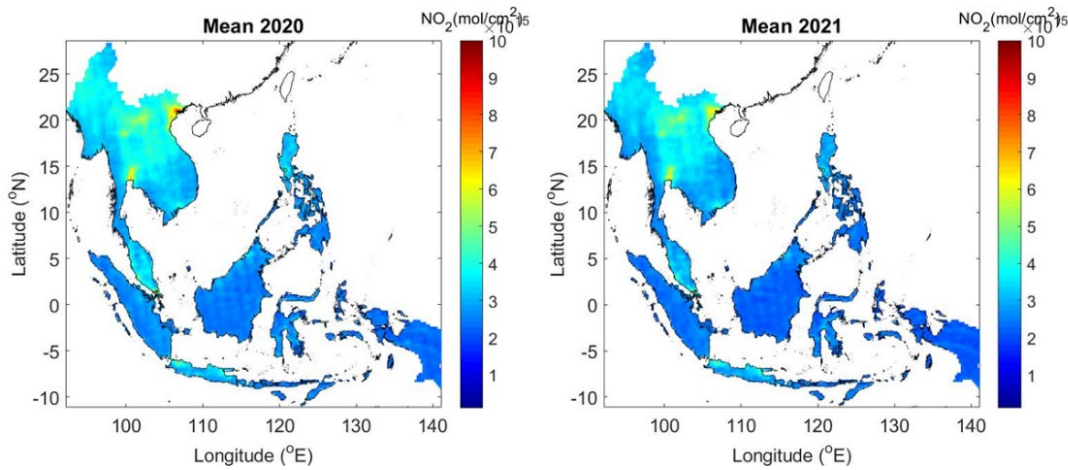
Figure 3. The average mean of Nitrogen Dioxide pollution in both 2020 and 2021.
