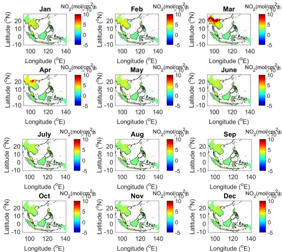
Figure 1. Nitrogen Dioxide pollution mapping for 2020.
